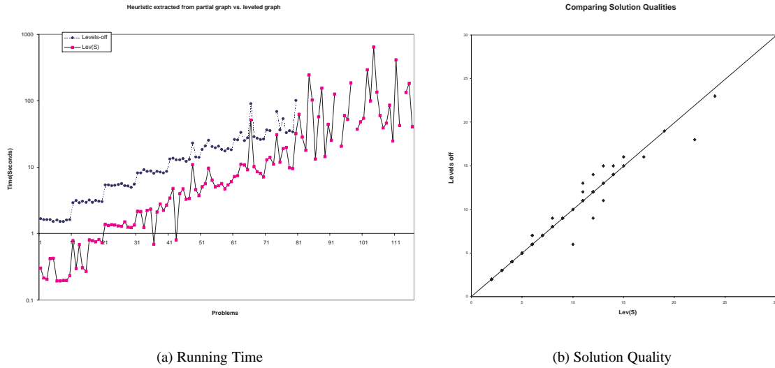
Figure 6: Results on trading heuristic quality for cost by extracting heuristics from partial planning graphs.
