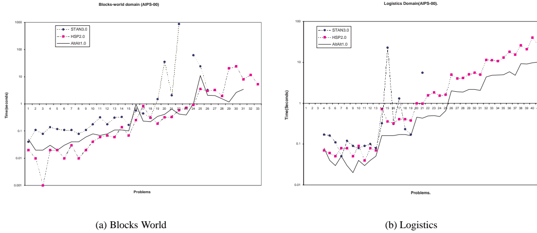
Figure 5: Results in Blocks World and Logistics
