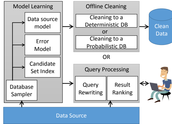
Fig. 1. The architecture of BayesWipe. Our framework learns both data source model and error model from the raw data during the model learning phase. It can perform offline cleaning or query processing to provide clean data.
