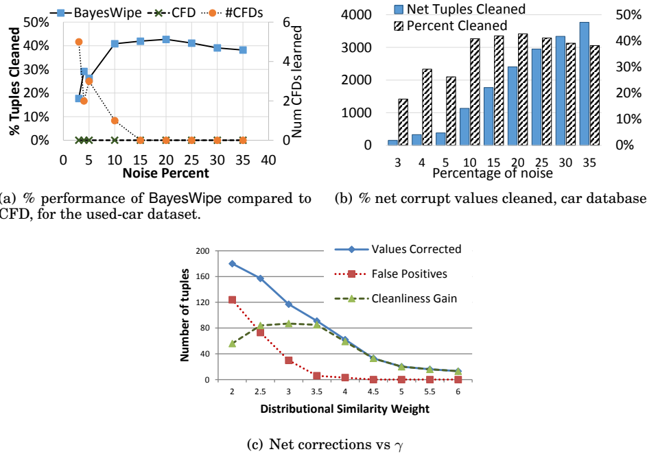
Fig. 6. Offline cleaning mode of BayesWipe
