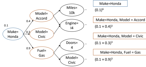
Fig. 3. Query Expansion Example. The tree shows the candidate constraints that can be added to a query, and the rectangles show the expanded queries with the computed probability values.
