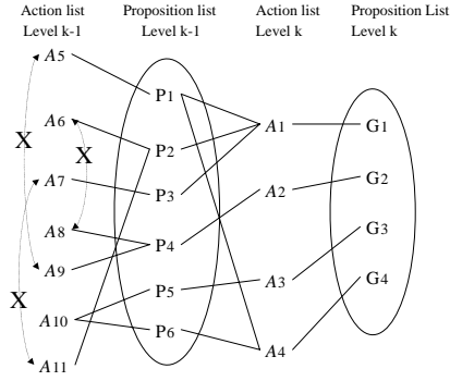
(a) Planning Graph
