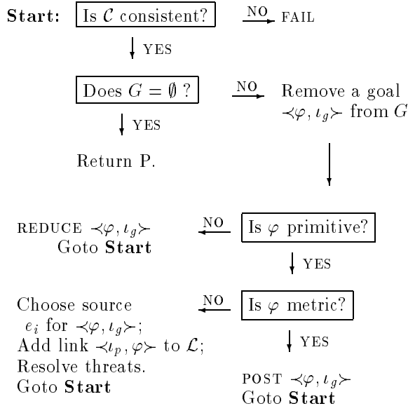
Figure 3: The main loop of ZENO.
