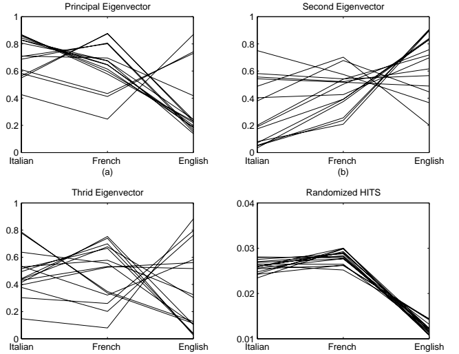
Figure 4: Results on random corpora.
